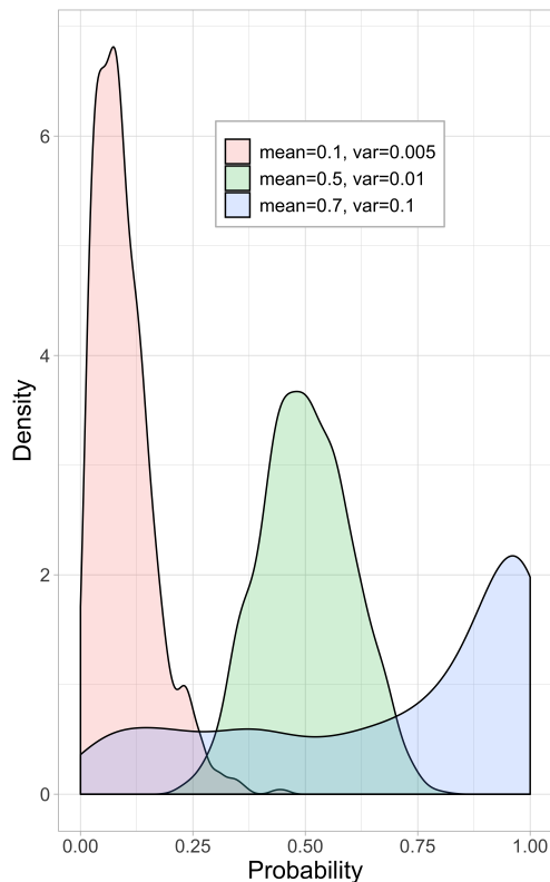
Figure 6: Fig. 6. Examples of probability densities for three different Beta distributions.
