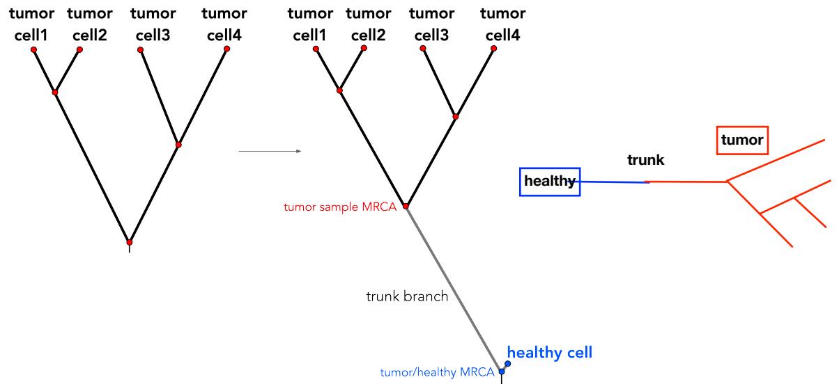
Figure 4: Fig. 4. Addition of a healthy cell in a tumor scenario. In this case we expect that the healthy cell has evolved much slower than the tumoral cells, so a small (or zero) outgroup might make more sense. In this example, the corresponding values were -k0.5 -q0.05 .
